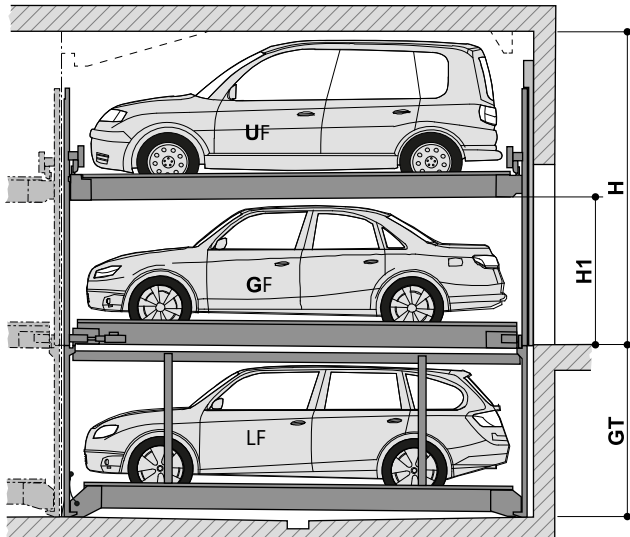
GT: Pit depth H: Building height H1: Headroom
