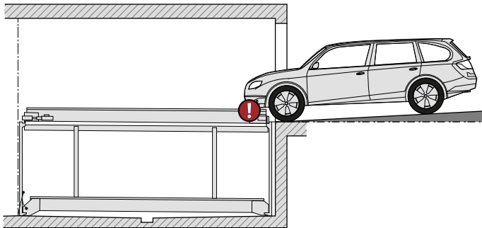
max. 3% slope
